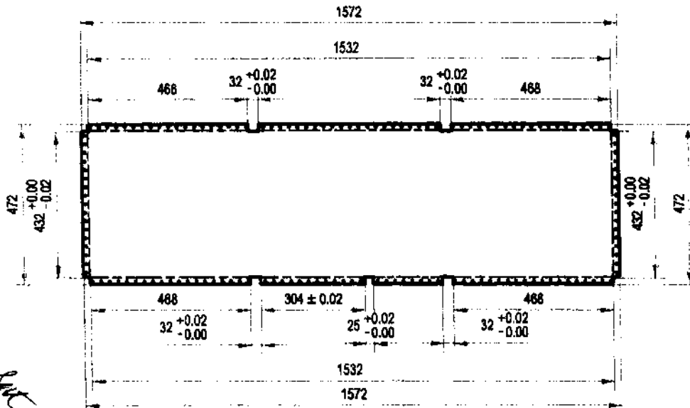
DETAIL A-1.2:
