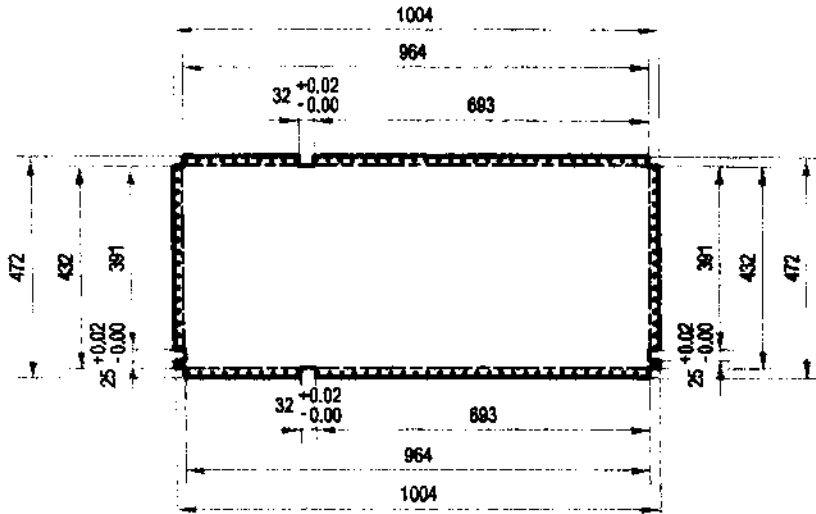
DETAIL A-4.1:
