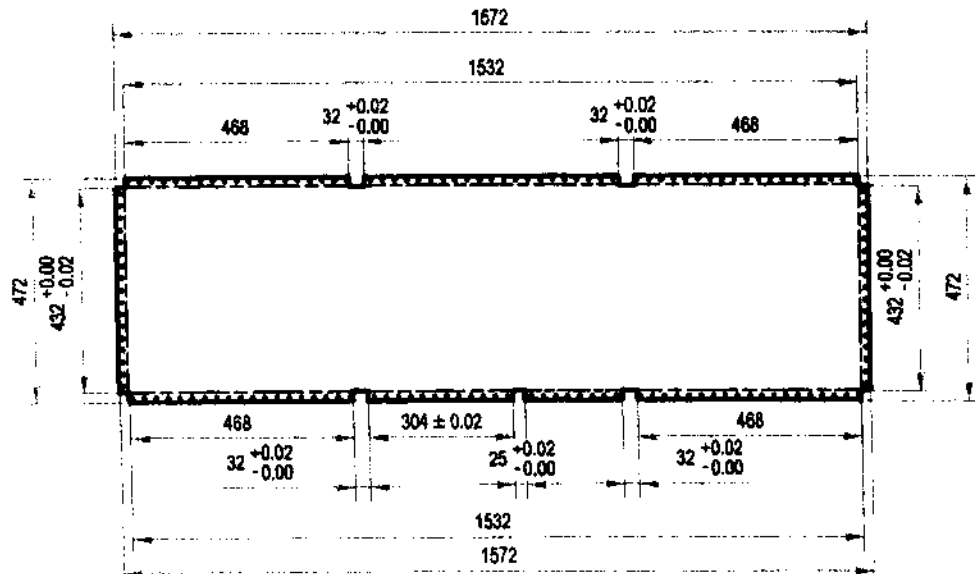
DETAIL A-1.2:
