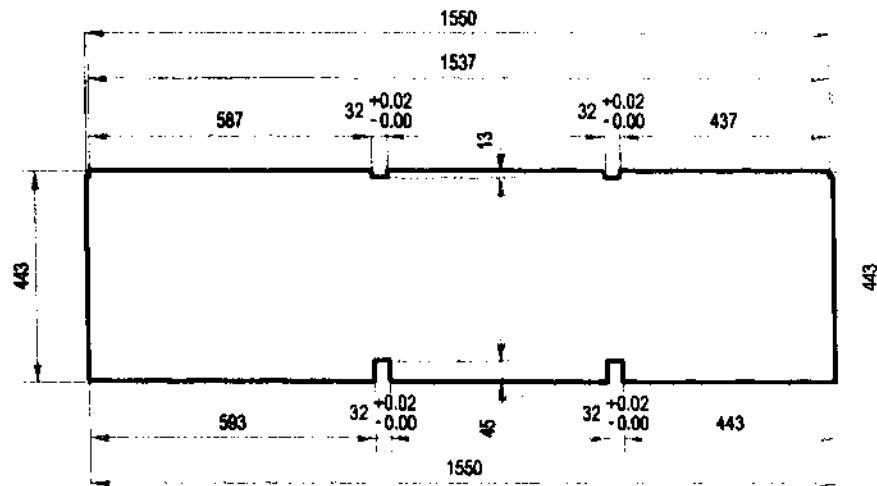
DETAIL A-5.4:
