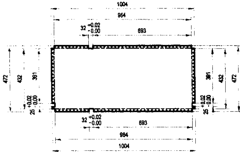
DETAIL A-4.1:
