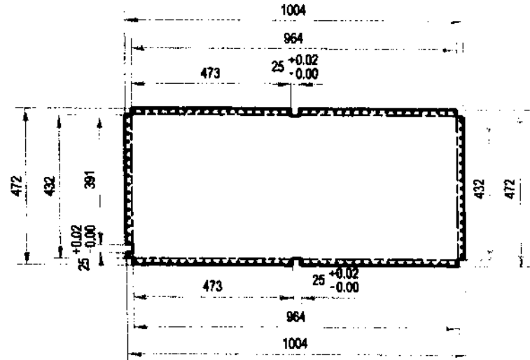
DETAIL A-3.4:
