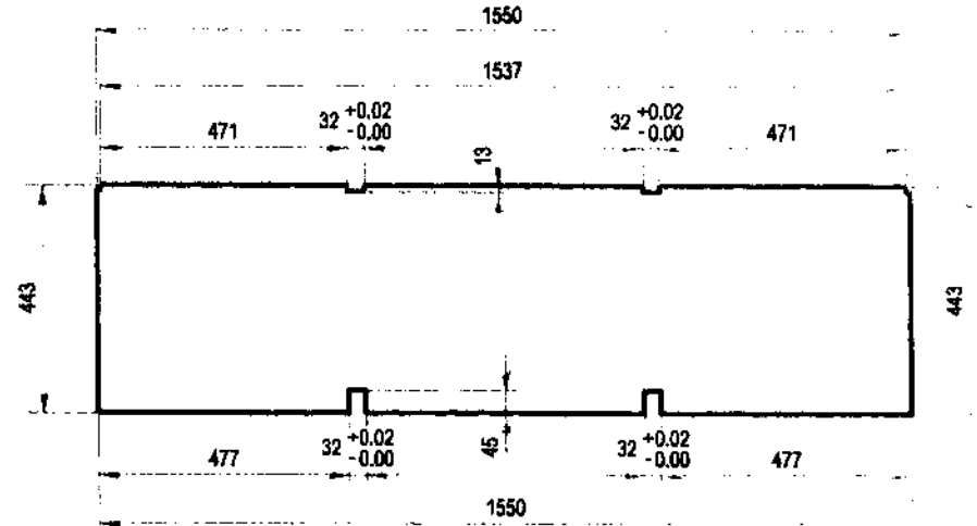
DETAIL A-5.3:
