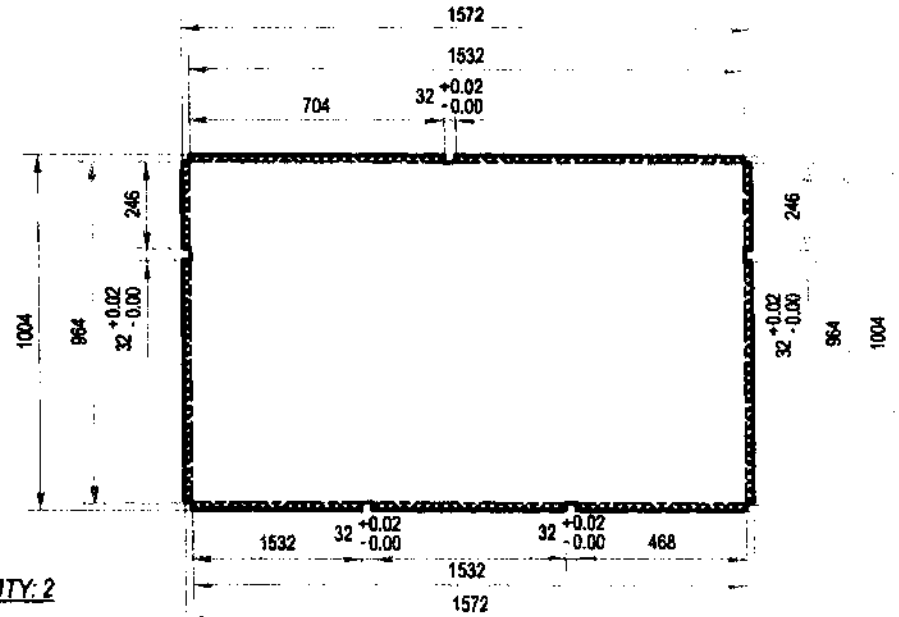
DETAIL A-2.4:
