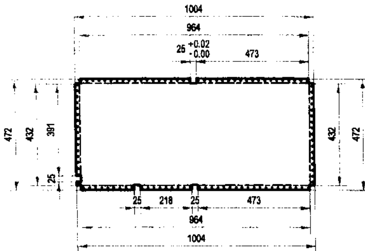
DETAIL A-4.2:
