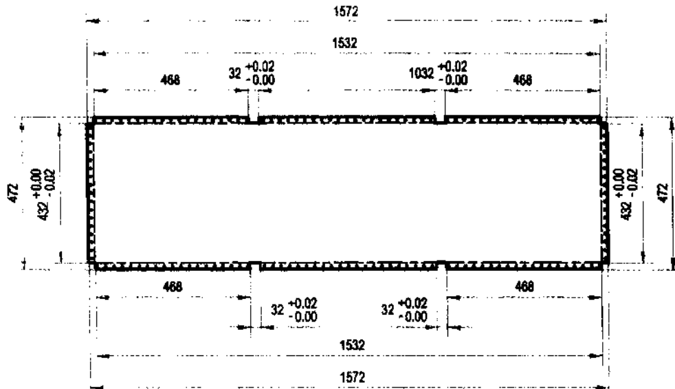
DETAIL A-1.1:
