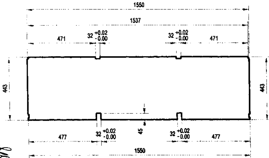
DETAIL A-5.2:
