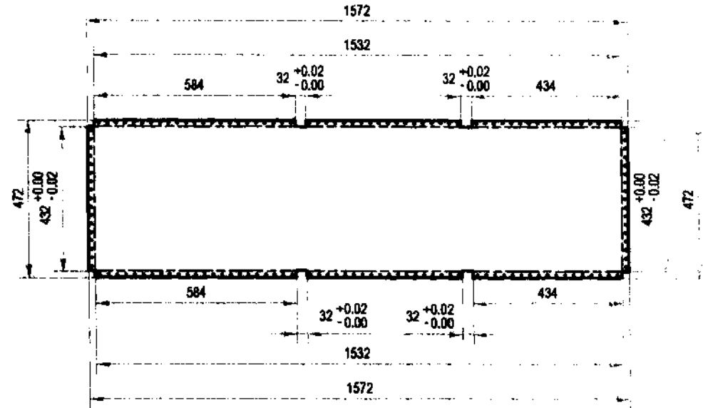
DETAIL A-1.3:
