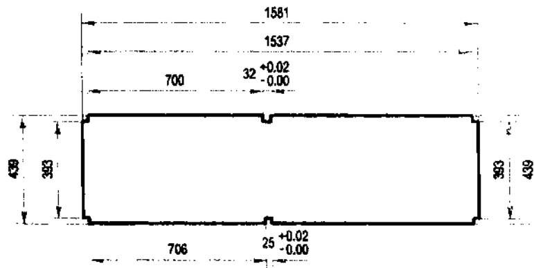
DETAIL B-1.4:
