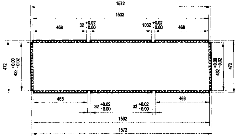
DETAIL A-1.1:
