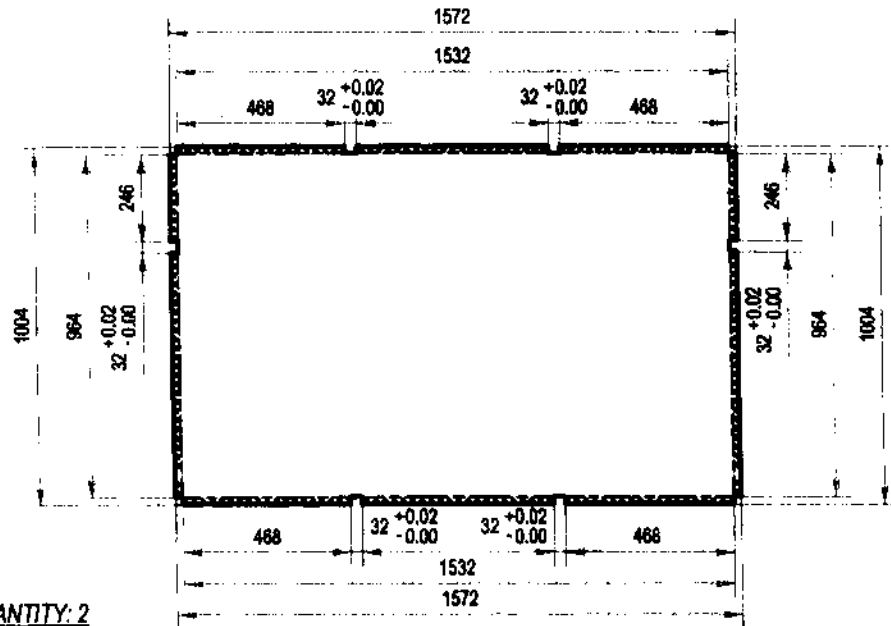
DETAIL A-2.2:
