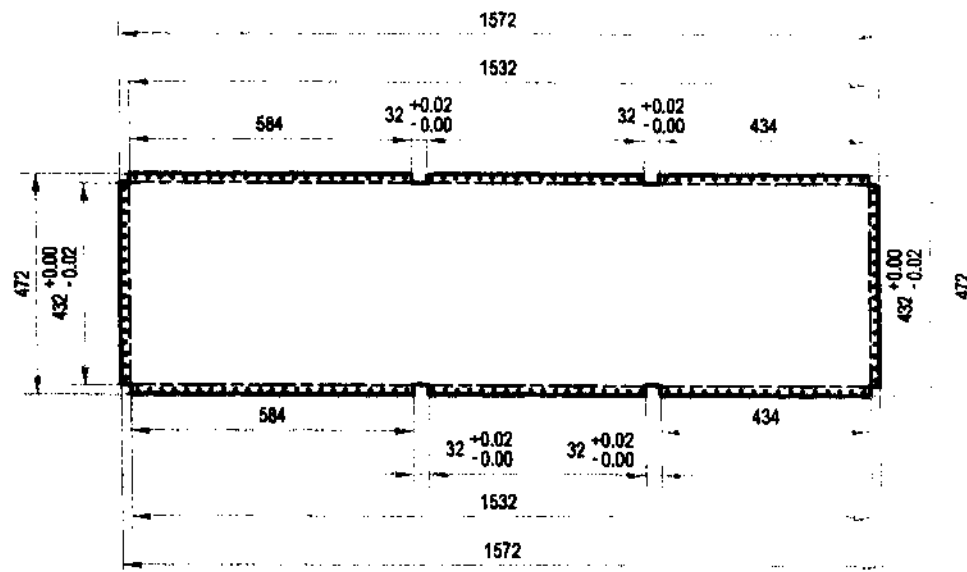
DETAIL A-1.3:
