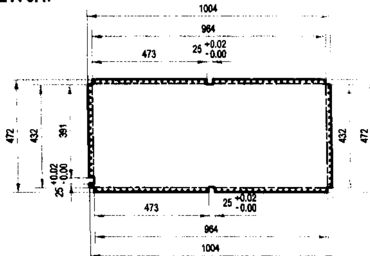
DETAIL A-3.4:
