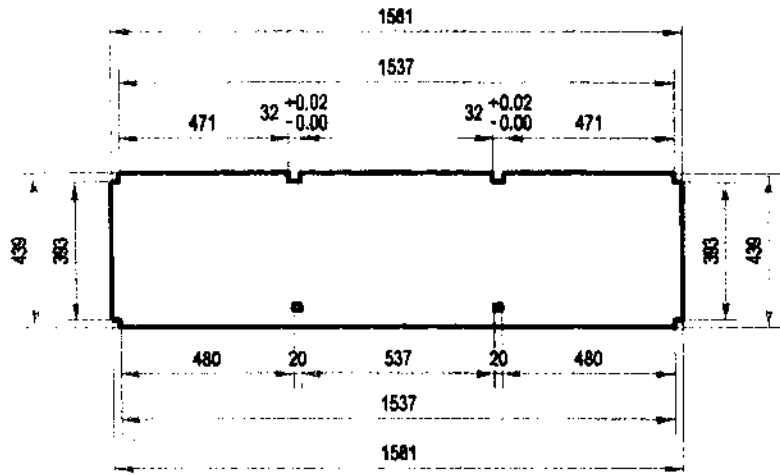
DETAIL B-1.1:
