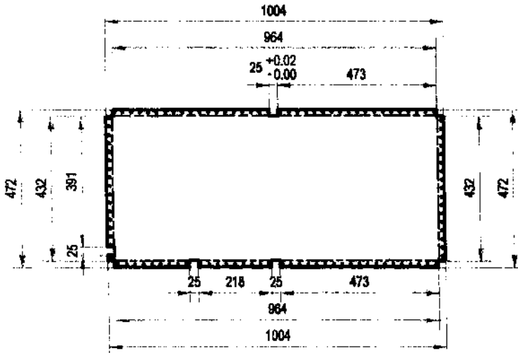
DETAIL A-4.2:
