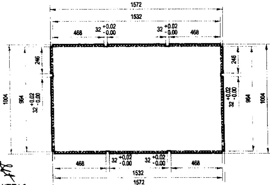
DETAIL A-2.2:
