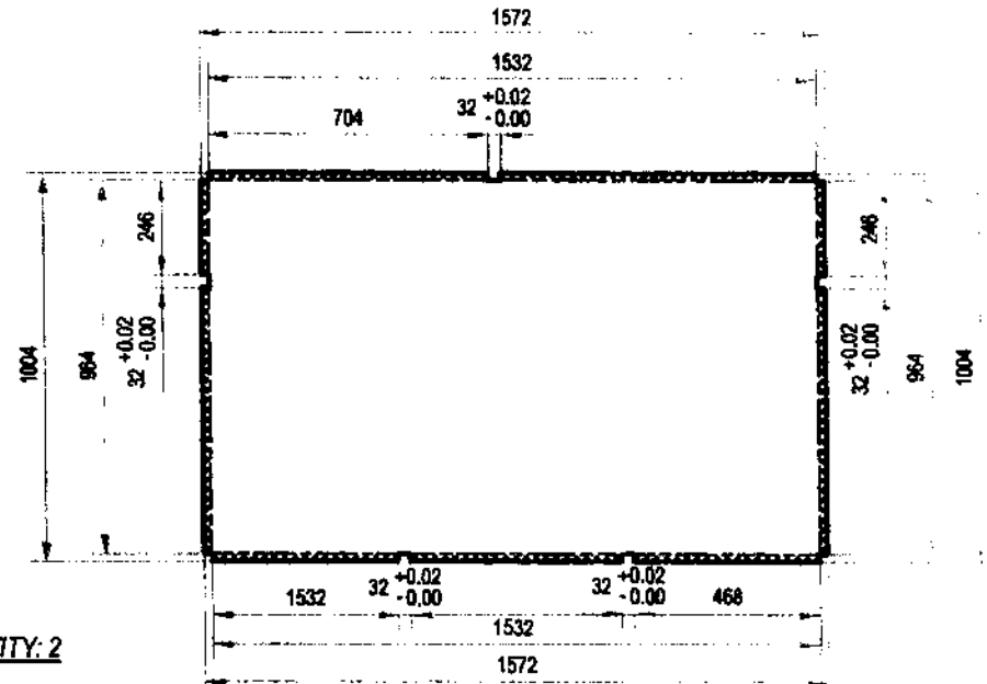
DETAIL A-2.4:
