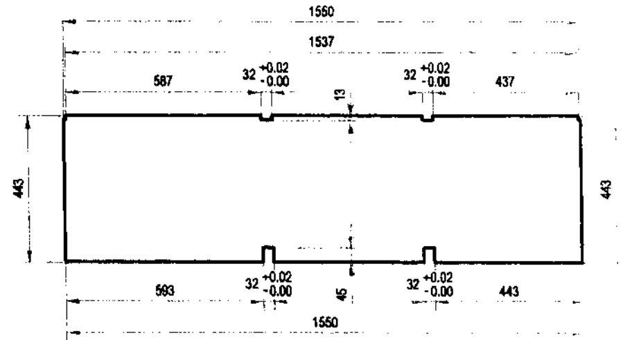
DETAIL A-5.4:
