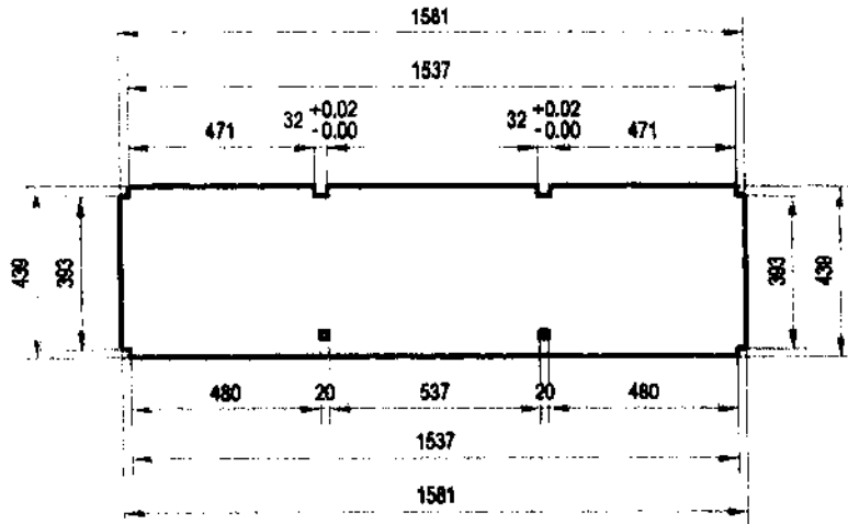
DETAIL B-1.1:
