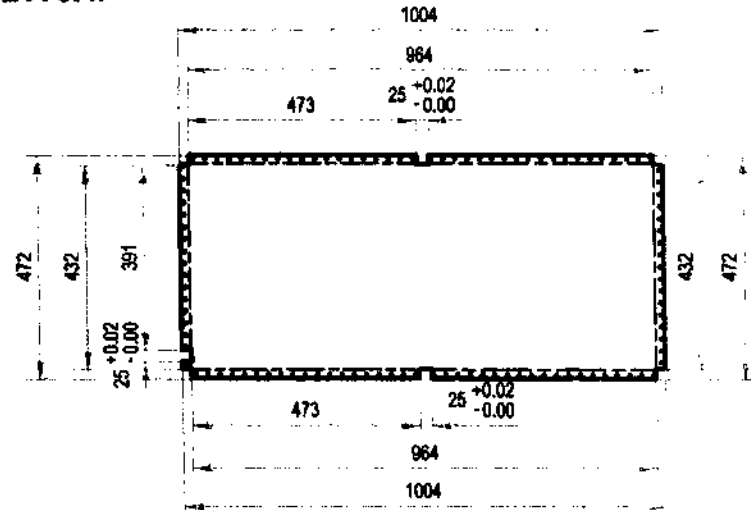
DETAIL A-3.4:
