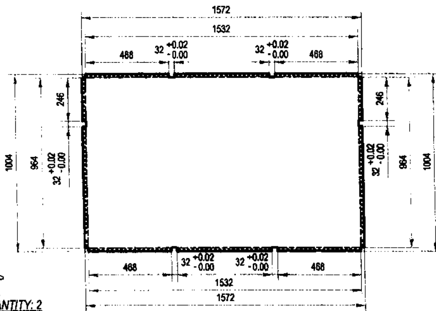
DETAIL A-2.2:
