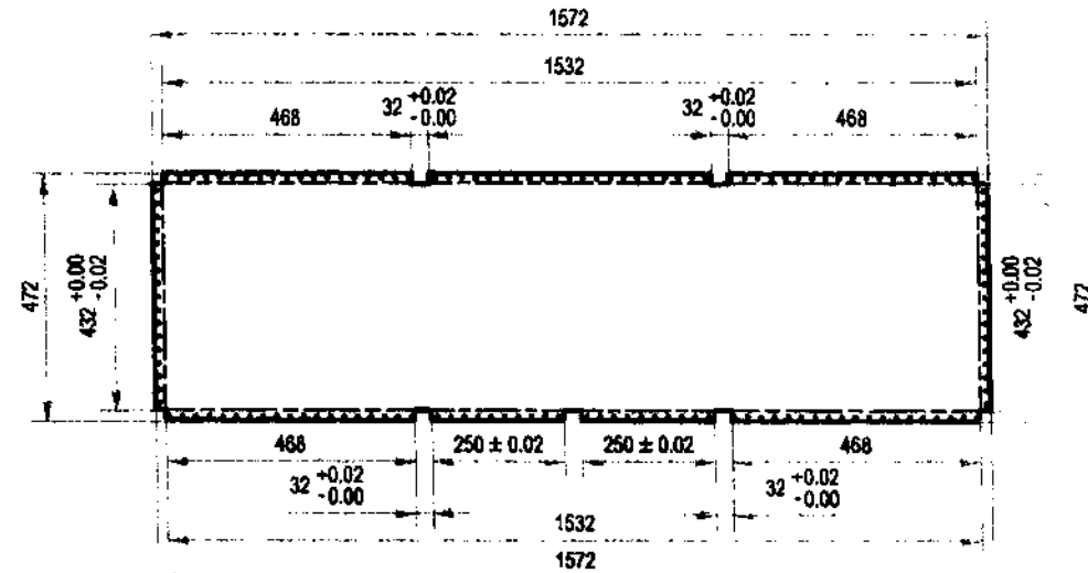
DETAIL A-1.4:
