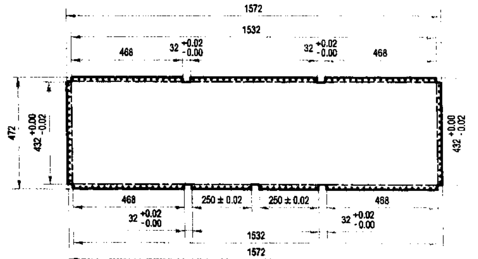
DETAIL A-1.4:
