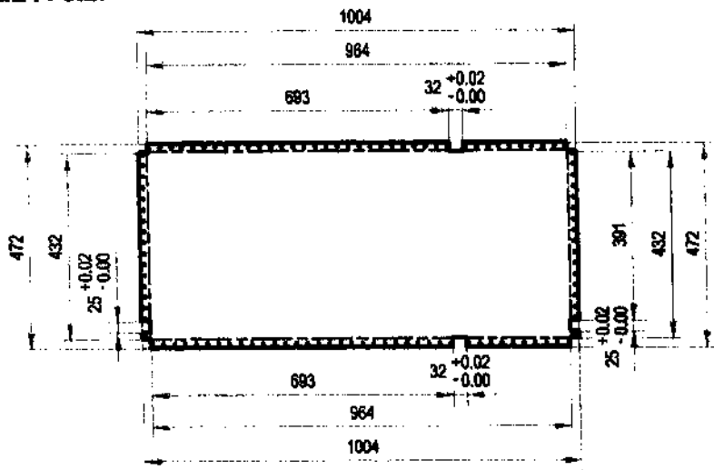
DETAIL A-3.2:
