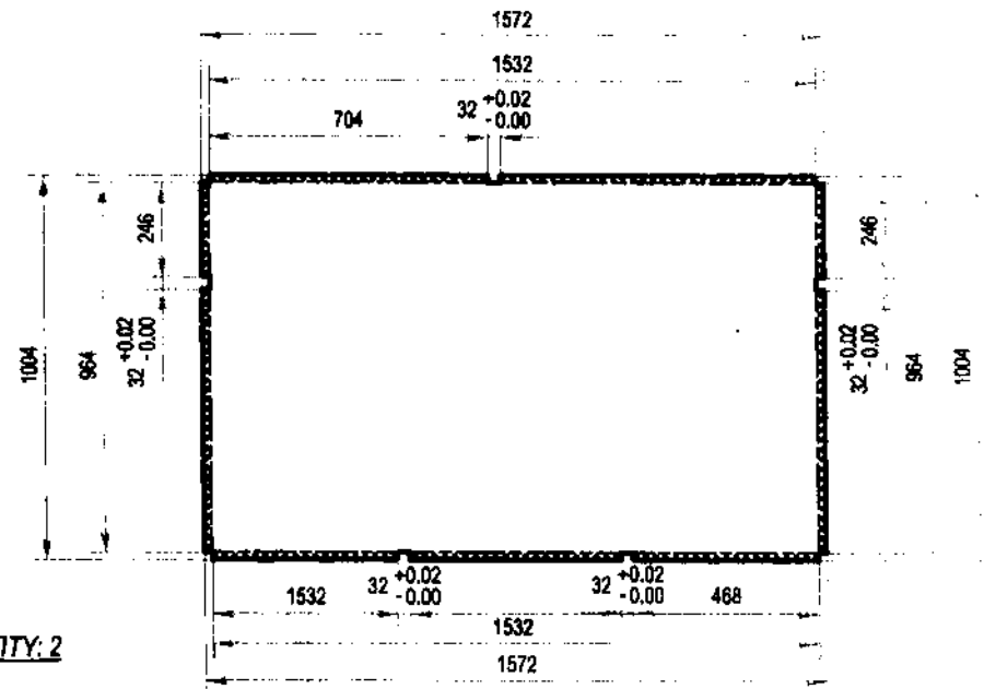
DETAIL A-2.4:
