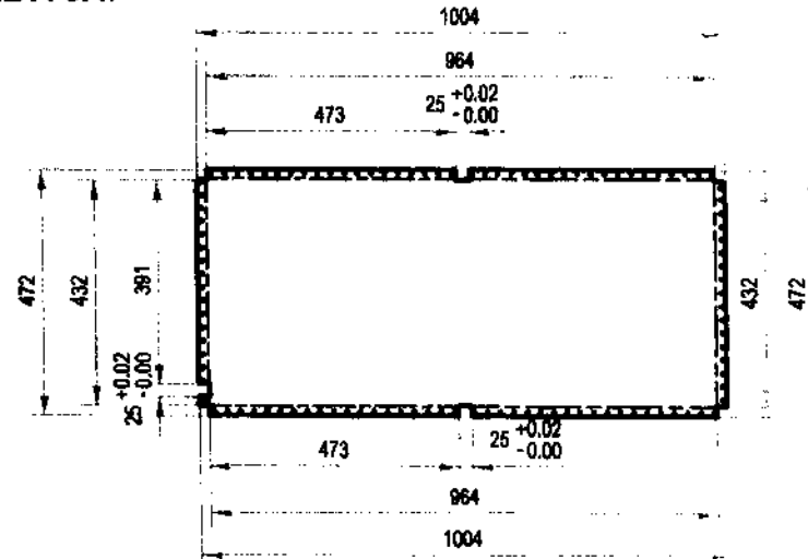
DETAIL A-3.4:
