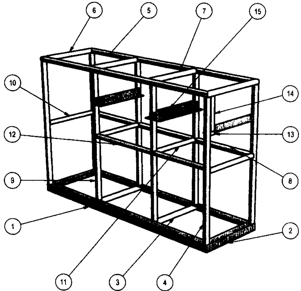
MTL BOX NO. 4 FRAME (BREAD AND PASTRY) (The door is not shown in the drawing)
