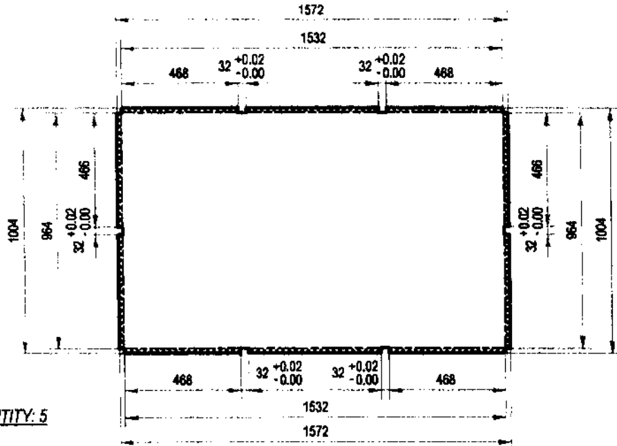
DETAIL A-2.2:
