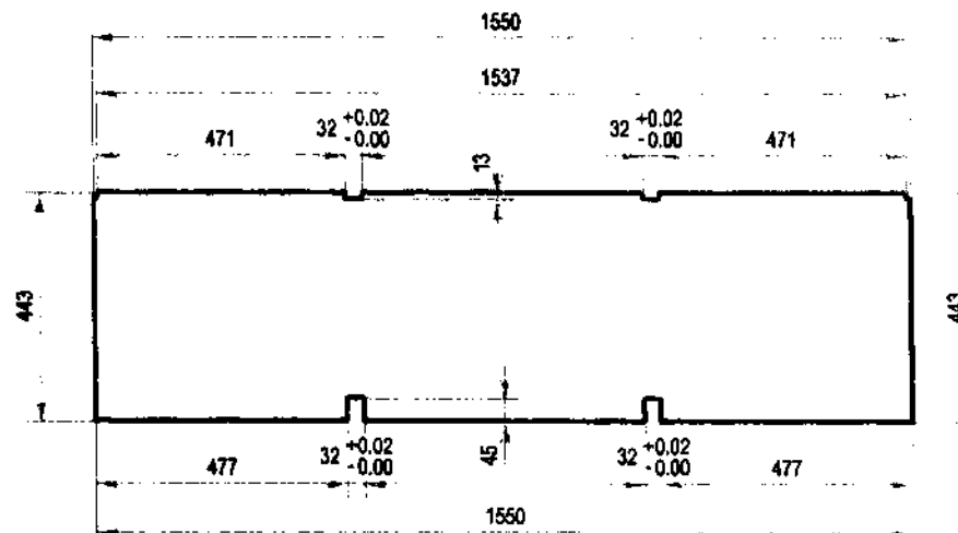
DETAIL A-5.3:
