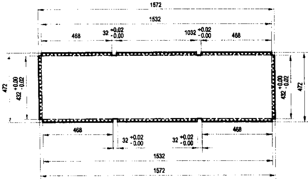
DETAIL A-1.1:
