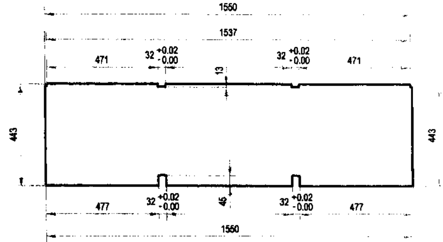
DETAIL A-5.3:
