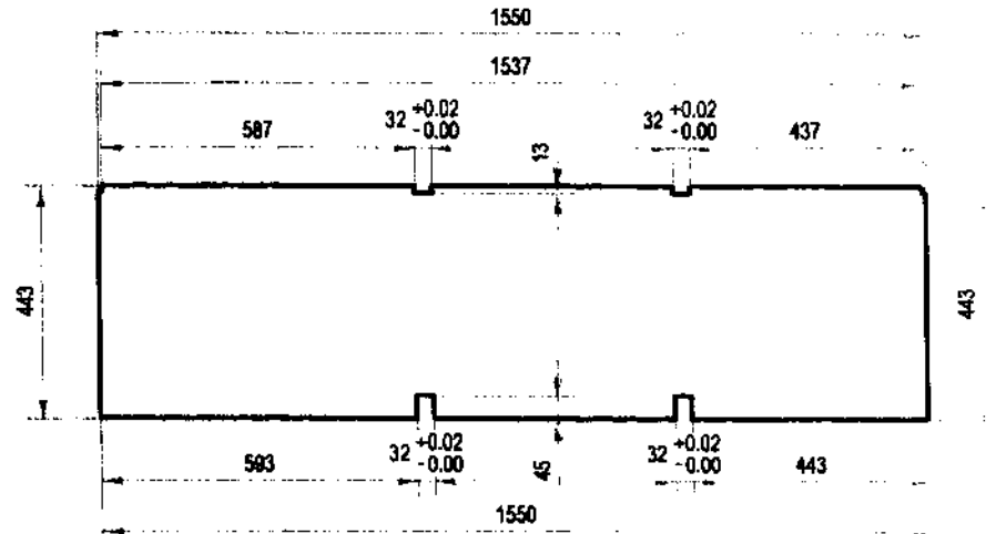
DETAIL A-5.4:
