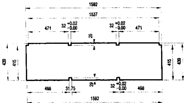
DETAIL B-1.2:
